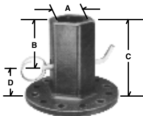
P630013 Kelly Bar Adapter
